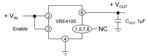
Figure 2 External Connections
